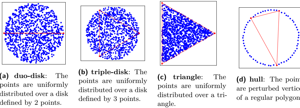
■ Figure 1 The 4 types of data-sets of the minimum enclosing disk problem used in our experimental evaluation: duo-disk, triple-disk, triangle, and hull
