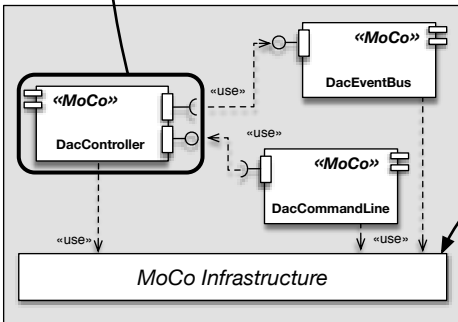
Component Architecture View (DAC-PL)
