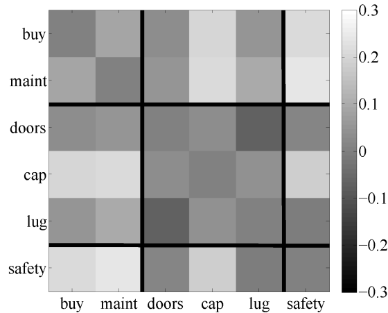
Figure 3: Visualization of the interaction index for the car evaluation data (numerical values are shown in terms of level of gray, values on the diagonal are set to 0). Groups of related criteria are indicated by the black lines.
