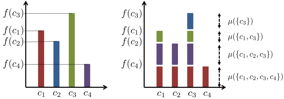
Figure 1: Vertical (left) versus horizontal (right) integration. In the first case, the height of a single bar, f(c_i) , is multiplied with its “width” (the weight \mu(\{c_i\}) ), and these products are added. In the second case, the height of each horizontal section, f(c_{(i)}) - f(c_{(i-1)}) , is multiplied with the corresponding “width” \mu(A_{(i)}) .
