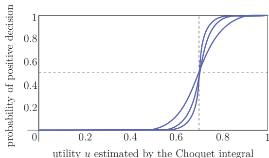
Figure 2: Probability of a positive decision, \mathbf{P}(y = 1 \mid \mathbf{x}) , as a function of the estimated degree of utility, u = U(\mathbf{x}) , for a threshold \beta = 0.7 and different values of \gamma .
